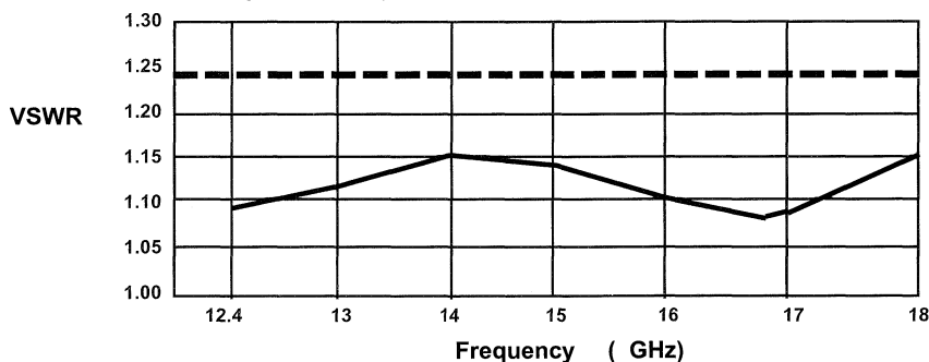
Typical Waveguide Adapter Performance Characteristics
