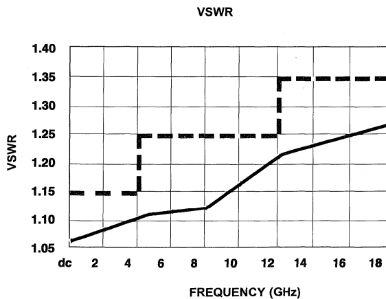
Typical Fixed Attenuator Performance Characteristics
