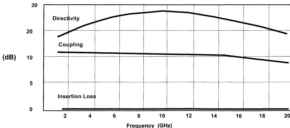
Typical Directional Coupler Characteristics
