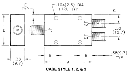
CASE STYLE 1, 2, & 3
