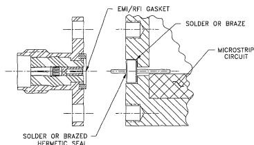
Drop-in Assembly - Flanged Connector
