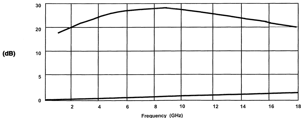
Typical Power Divider Characteristics
