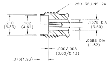
Female Jack
