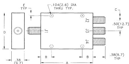
CASE STYLE 1
