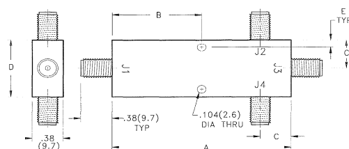
CASE STYLE 2
