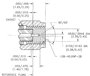
Male Plug
