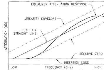
Negative Slope Equalizer Response
