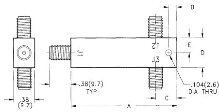
CASE STYLE 4
