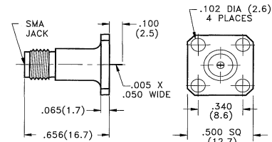
Figure 1 - non- removable tab contact
