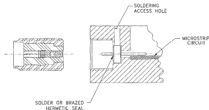
Drop-in Assembly - Feedthru Connector
