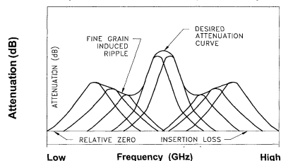
Multiple Section Fine Grain Equalizer Response
