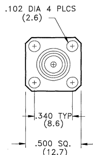
Typical End View - All Models
