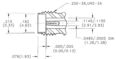
Female Jack
