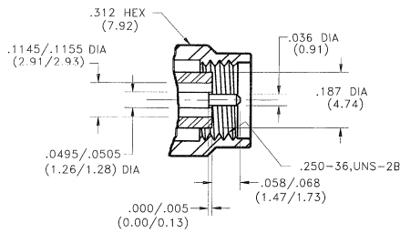
Male Plug
