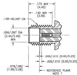
Female Jack
