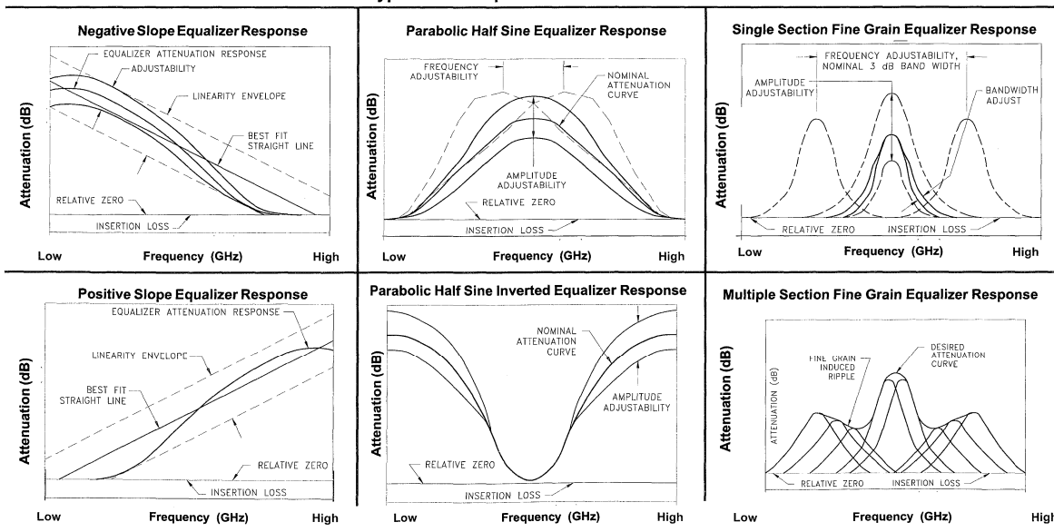
Typical Gain Equalizer Characteristics
